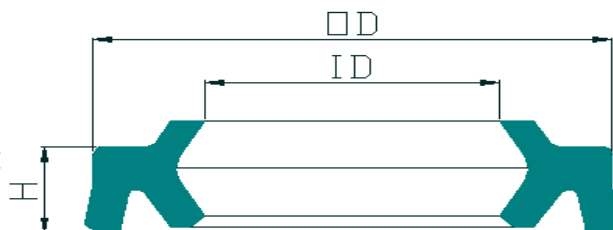
TYPE - WH3
